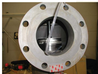
Figure 2: Location of test probe in EPA Method 21 test setup located directly at sealing surface
